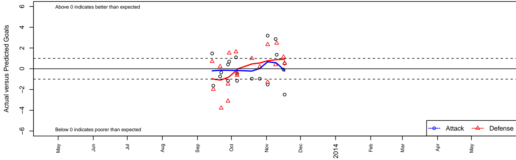
The Academy Cads G02 Dots are actual minus expected GF (blue circles) and GA (red triangles). Blue line is smoothed change in attack strength. Red is smoothed change in defense strength.
